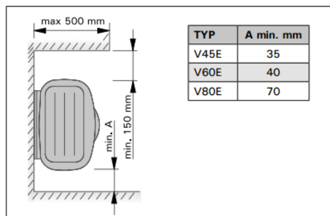
Figure 9. Installation of the heater in a recess
