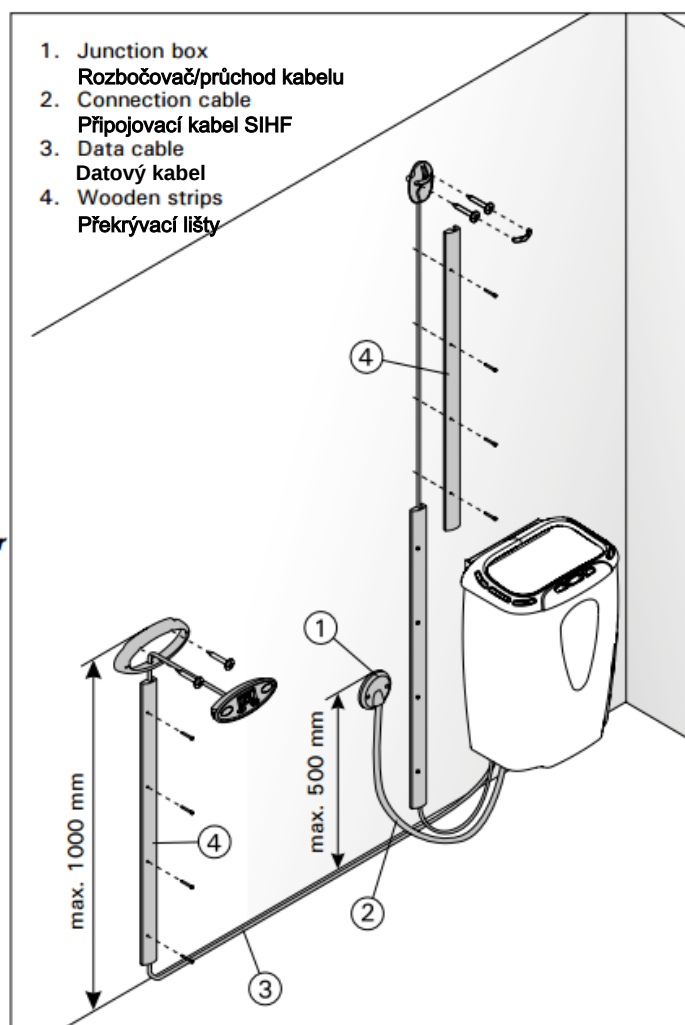
Figure 10. Connections of the heater
