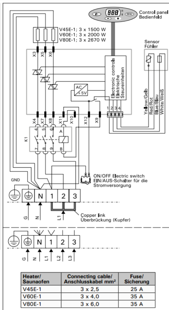
Figure 11b. 1/3 phase electrical connections of heater V45E-1, V60E-1, V80E-1
